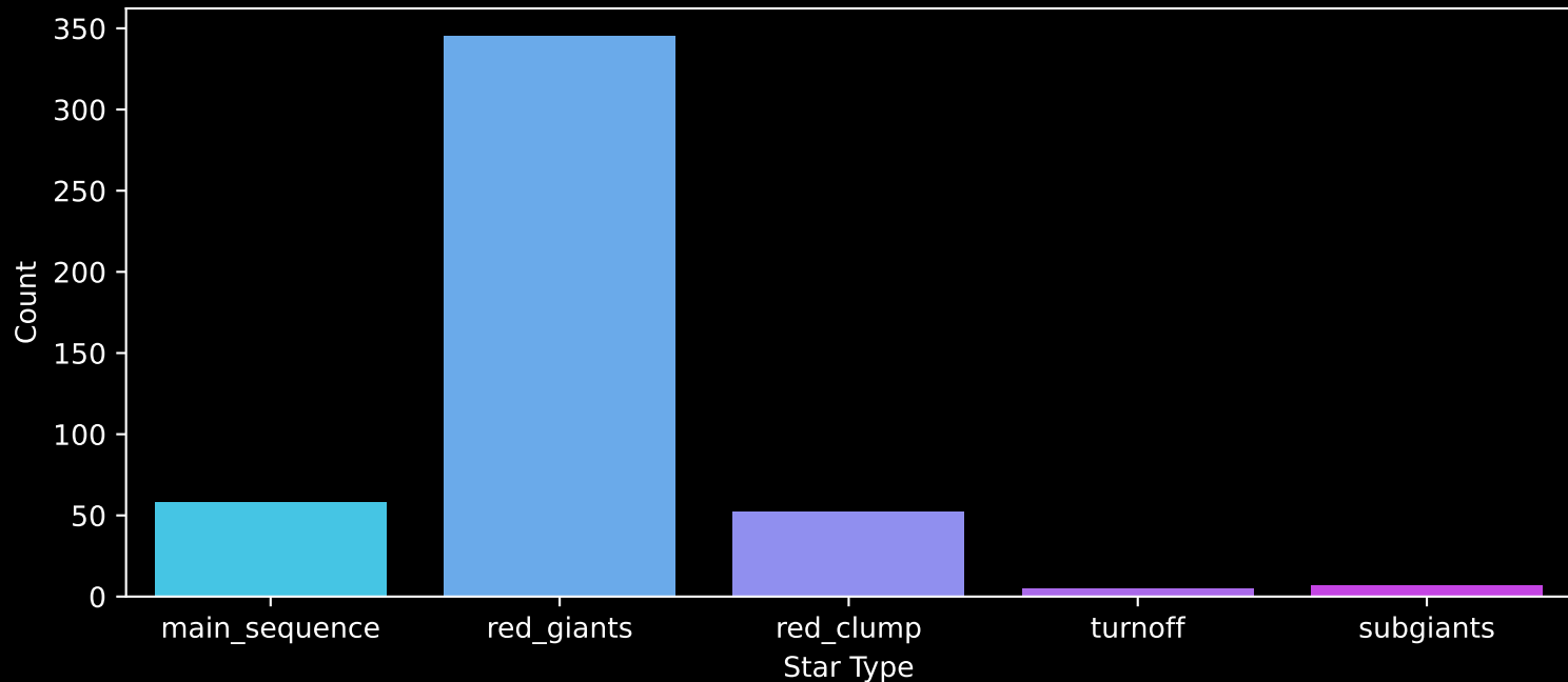
APOGEE DR17 Field: [240+08] Count plot of Star Type
