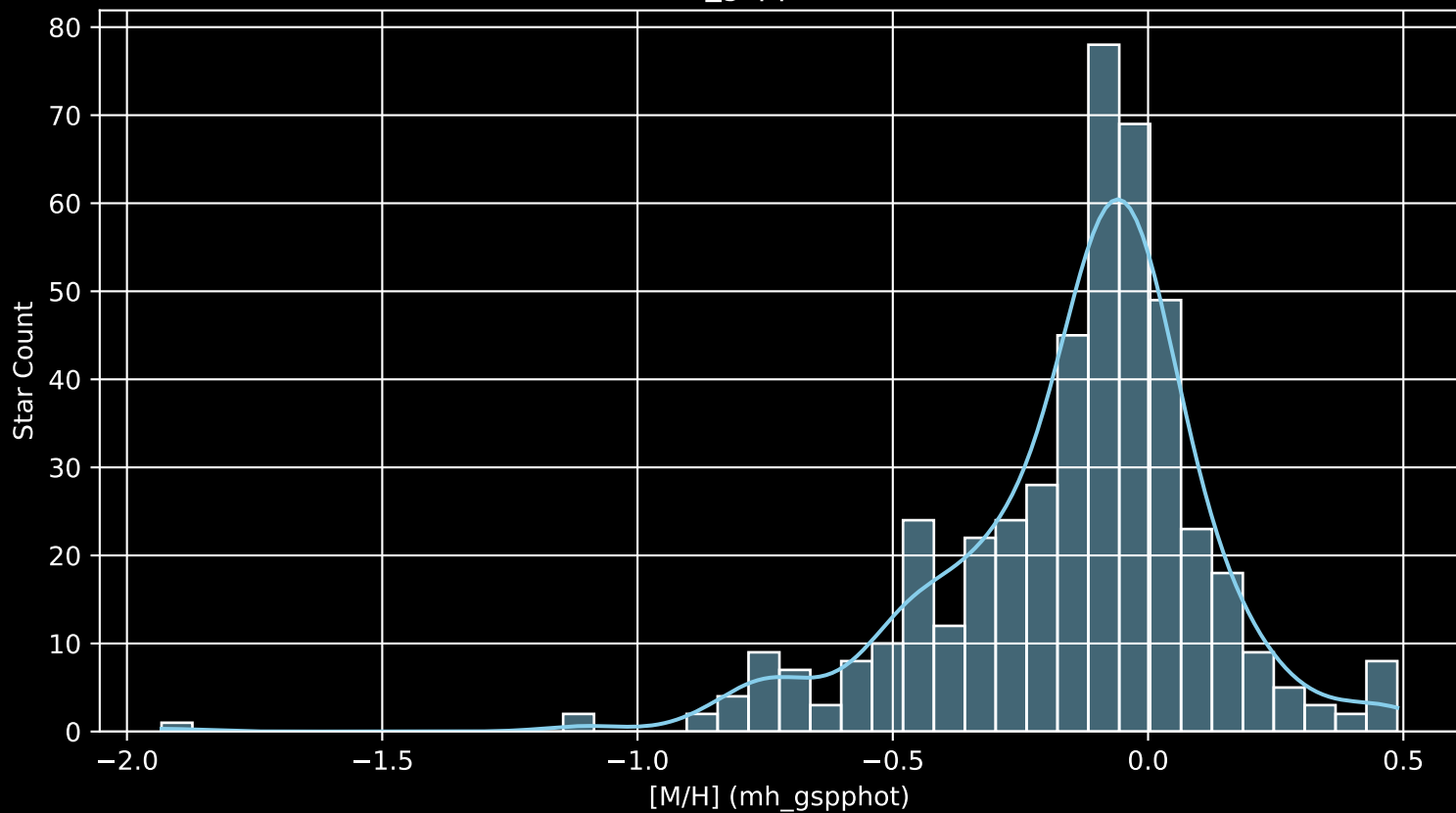
APOGEE DR17 Field: [240+08 [M/H] (mh_gspphot) (n= 465)
