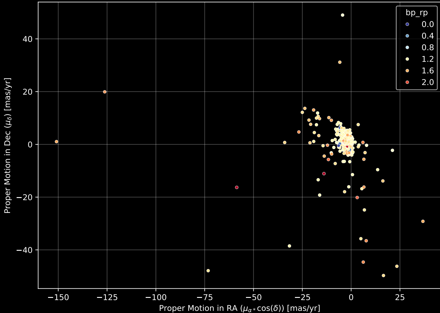
APOGEE DR17 Field: [240+08] Proper Motion Diagram (n= 467)
