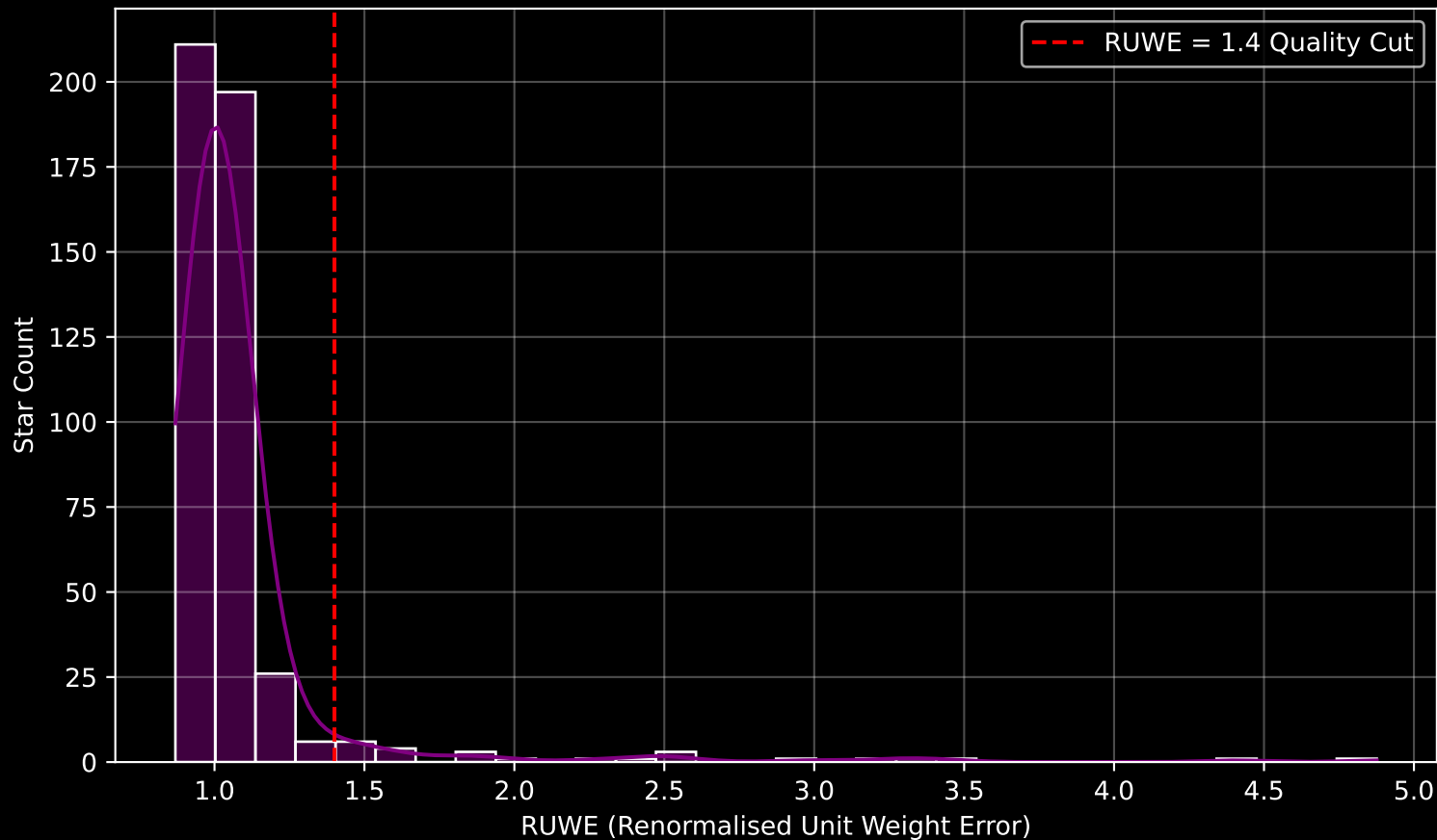
GAPOGEE DR17 Field [240+08] RUWE Distribution (n= 465)
