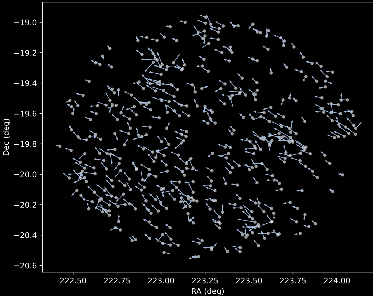
APOGEE DR17 Cluster 1 Proper Motion Vectors (n=422)
