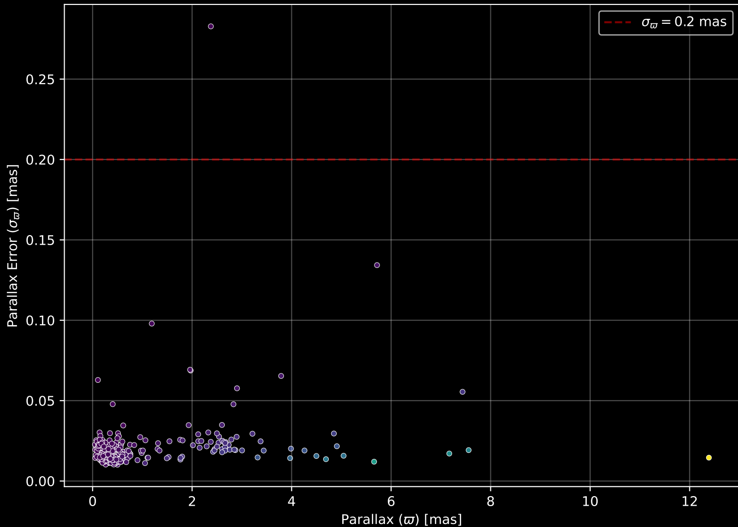
APOGEE DR17 Field: [240+08] Parallax Quality (n= 467)
